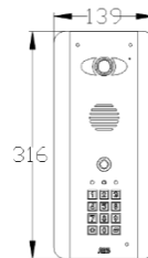
PRED2-WiFi-FSK/FBK Call Panel
